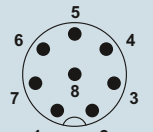
Pin, 8-pos., A-coded
